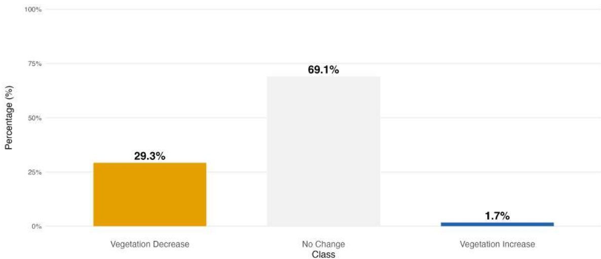
Figure 5.2: NDVI change map and NDVI change distribution in the Pra River Basin between 2018 and 2022.
